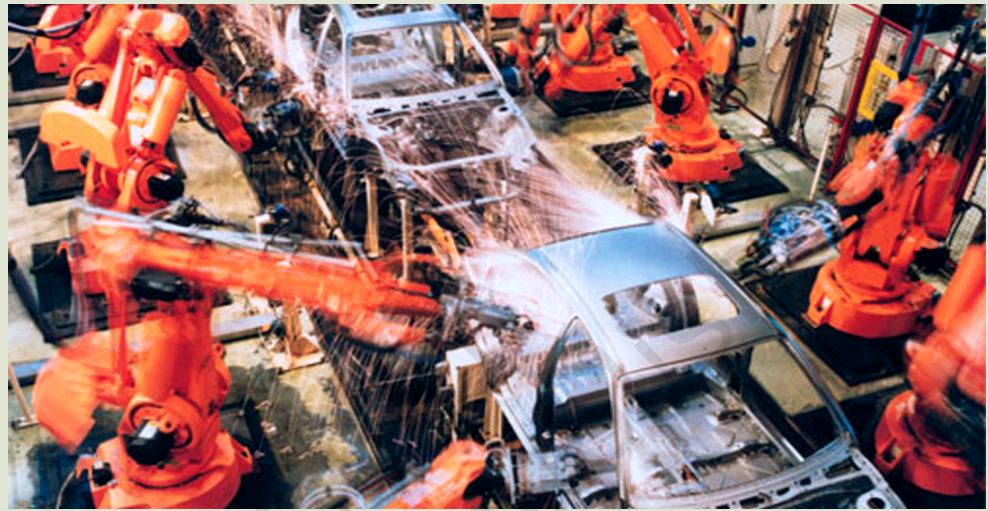
Figure 14.6 : Robot welding the car body
