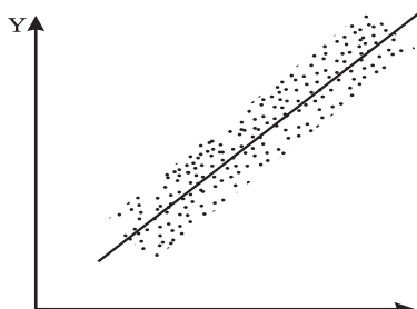
Fig. 7.1: Positive Correlation
