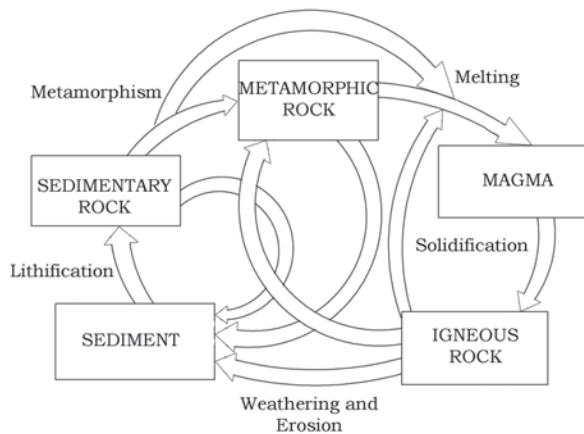
Fig 5.1 : Rock Cycle
