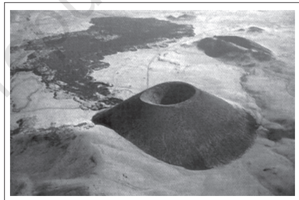
Shield Volcano
