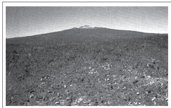
Cinder Cone
